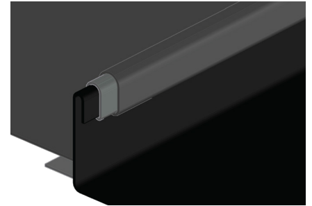
Double lock Panel
